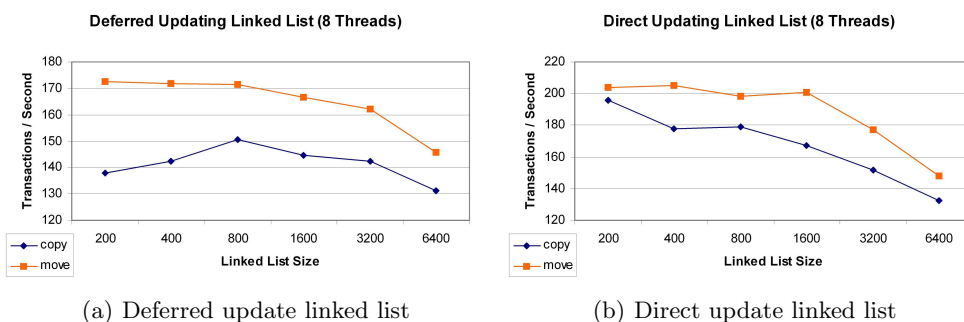
Fig. 1. Linked list benchmarks.
